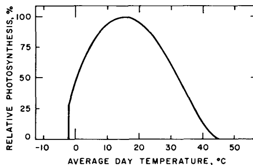
FIG. 3. The temperature response curve of the photosynthesis model assuming constant light and a 12-h day. An efficiency of 1 was assigned at the highest point on the curve.
