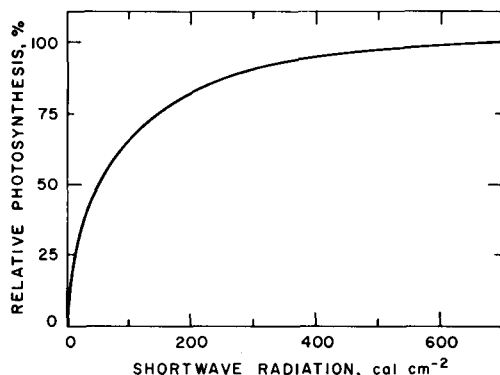
FIG. 2. The light response curve of the photosynthesis model assuming constant temperature and a 12-h day. An efficiency of 1 was arbitrarily assigned at 700 cal cm -2 day -1 (1 cal cm -2 min -1 = 69.8 mW cm -2 min -1 ).
