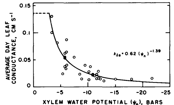
FIG. 4. The relation between average day leaf conductance ( k_{1a} ) of current year's foliage and xylem water potential at night ( \Psi_n ). Each point was the average of several leaf conductance measurements taken throughout the day. The parameters of the equation were arrived at by a least-squares-curve fit of the allometric function ( 1 \text{ bar} = 10^5 \text{ Pa} ). Data from Running (1976) and Emmingham (1974).
