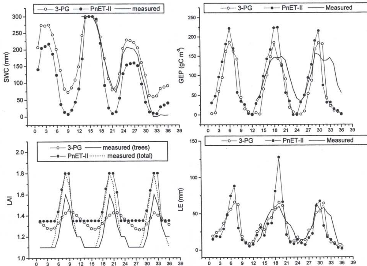
Fig. 2 Monthly comparisons of modelled and measured (a) soil water content (SWC, mm) (b) leaf area index (m 2 leaf m -2 ground, projected; dotted line is total LAI of understory and trees) (c) gross ecosystem production (GEP, g C m -2 month -1 ), and (d) water vapour exchange (LE, mm month -1 ) using the 3-PG and PnET-II models. Months 1–12 are for the last year of the 15–20 years equilibration of the models with the mean of 1996 and 1997 climate data. Months 13–24 are for 1996 climate, and months 25–36 are for 1997 climate (1996 and 1997 were run sequentially). ‘Measured’ soil water content was calculated from a simple one-dimensional water balance approach using the difference between measured precipitation and LE, and accounting for runoff when soil water content reached saturation. The model results are for soil water holding capacity set to 300 mm.
