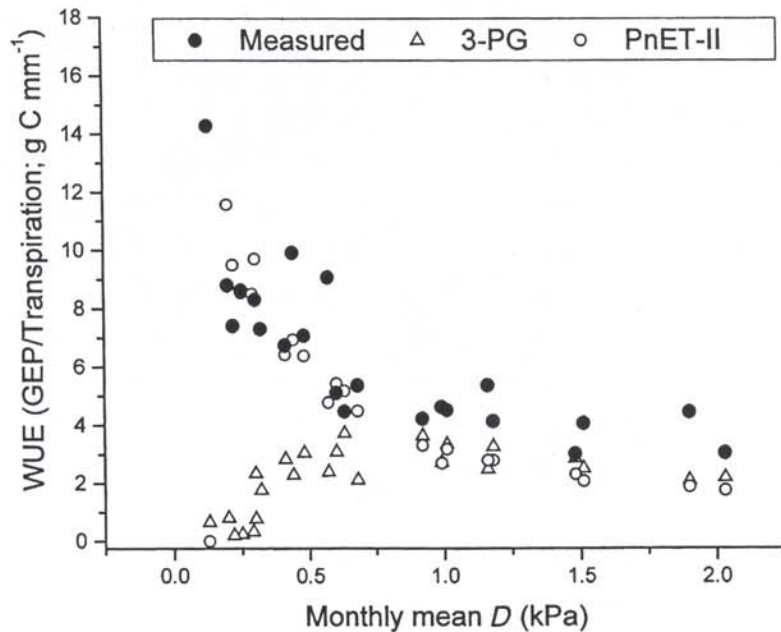
Fig. 4 Measured and modelled water use efficiency (WUE = GEP/transpiration) vs. monthly mean daytime D . Measured GEP was calculated from eqn (1), and transpiration was calculated from the seasonal fraction of above-to below-canopy LE.
